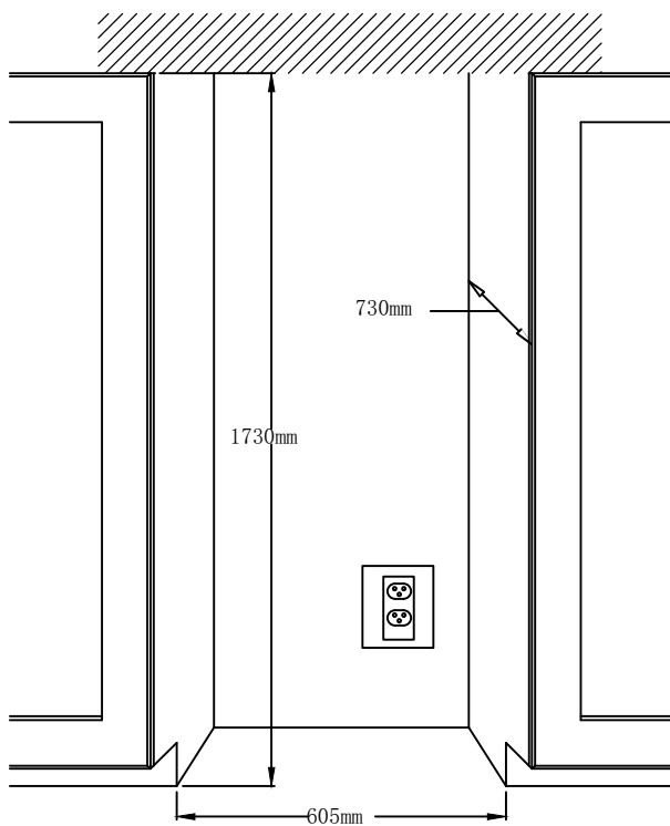
Cabinet Cut-Out
