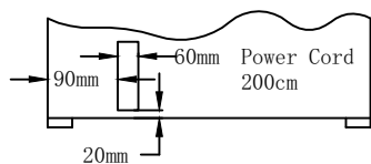
Cabinet Cut-Out
